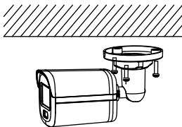
Figure 2-2 Secure the Camera to the Ceiling
