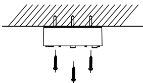
Figure 2-30 Secure the Junction Box Body
