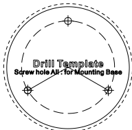
Figure 2-7 Drill Template
