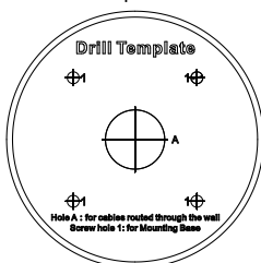
Figure 2-17 Drill Template
